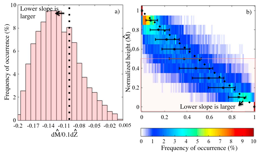
Figure 9. (a) Distribution of the normalized updraft mass flux profile slope in the lower half of the cloud layer. (b) Joint probability function of normalized updraft mass flux per normalized height. Included are the 0.1 slope (dotted line), the normalized updraft mass flux median (circle), and the interquartile range (whiskers) at each normalized height.
